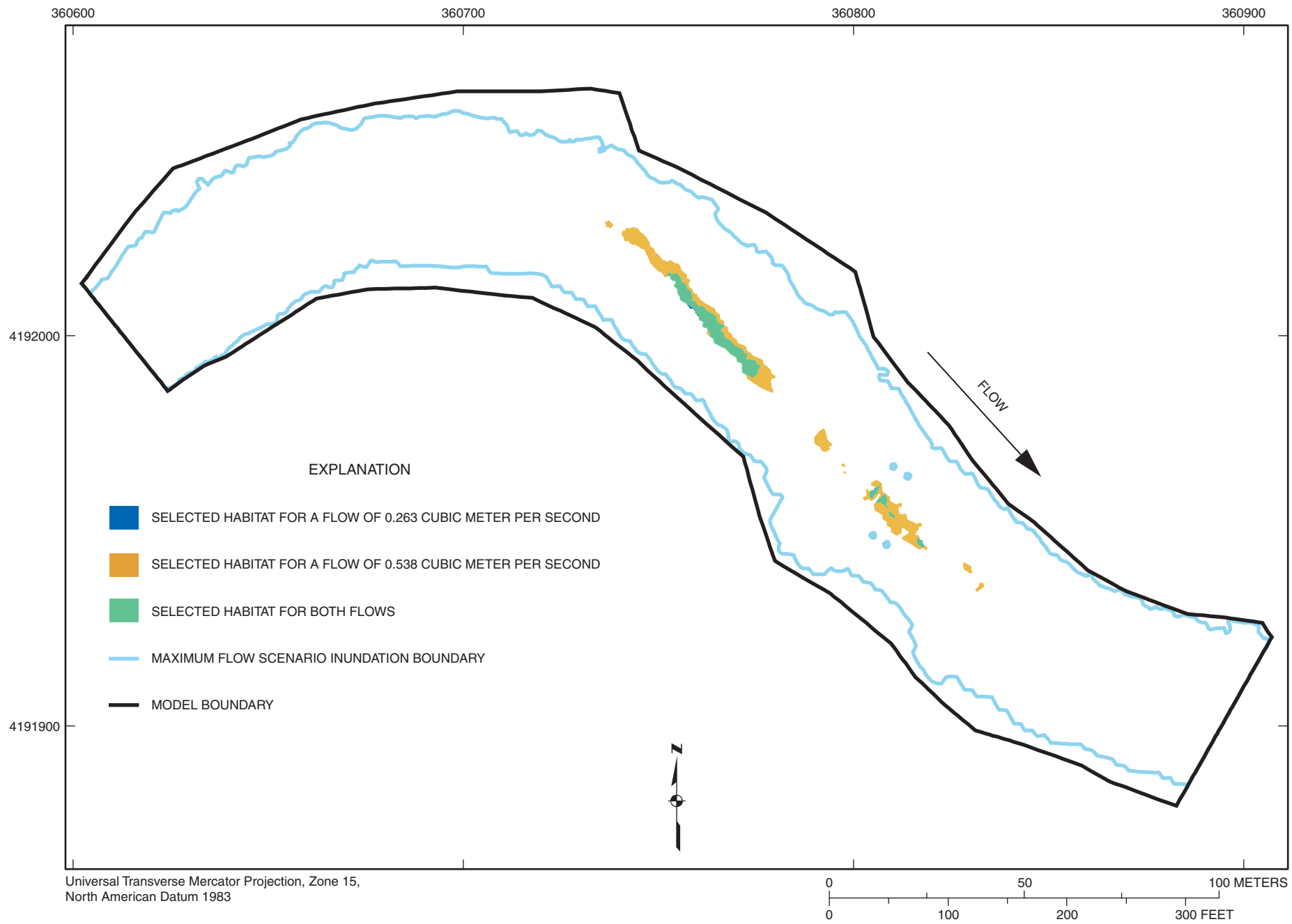
Figure 1-29. Selected habitat area distribution for habitat category 14 (flathead catfish) at flows of 0.263 and 0.538 cubic meter per second at Marmaton River site M1.
